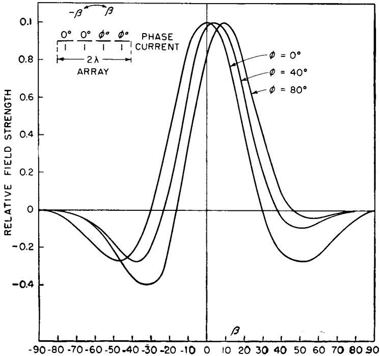
FIG. 3.47. Slew beam patterns for a row of four horizontal dipoles.
